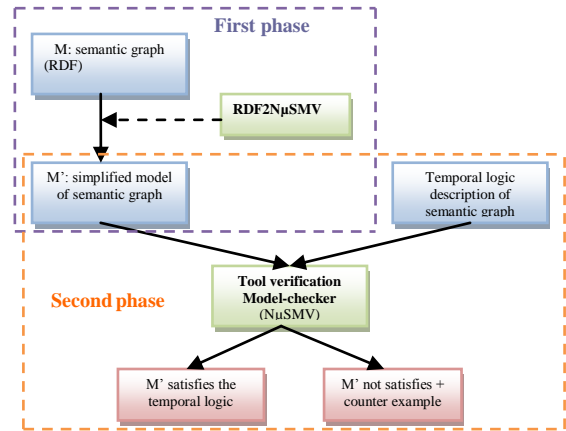
Figure 5. Our architecture.
