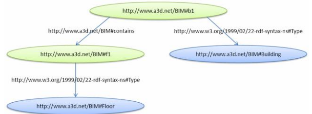
Figure 6. Example of partial RDF graph.
