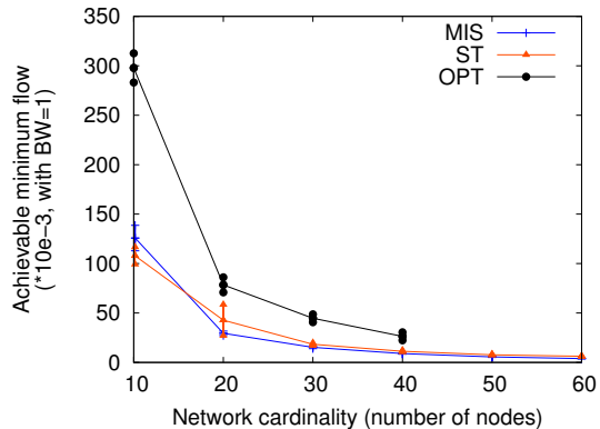
Fig. 4. Capacity (min-flow objective) for varying network cardinality
