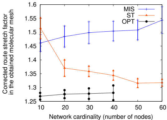
Fig. 3. Route stretch factor for varying network cardinality
