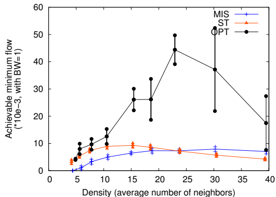
Fig. 5. Capacity (min-flow objective) for varying density
