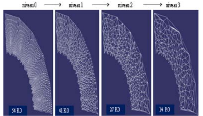
Figure 8 : example of two fragments simplification with maximum radius of curvature = 120^\circ .
