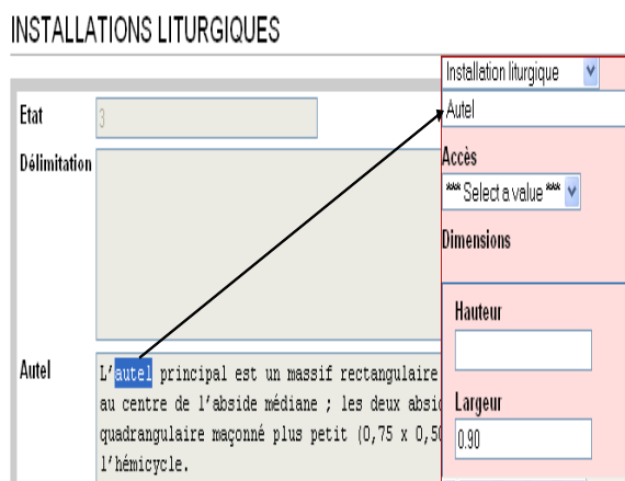
Figure 6: Annotation interface.
